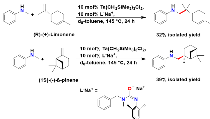
Figure 1. Reaction scheme for \beta -pinene and limonene amination by hydroaminoalkylation. 3
