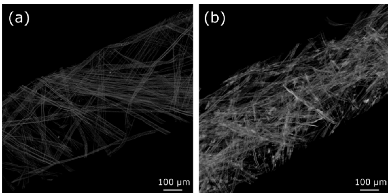
Figure 2. 3D reconstructed \mu CT image of a paper handsheet prepared with (a) unlabelled, (b) Fe-labelled fibres. The analysis revealed that Fe particles distributed through the sample enhance the contrast for fibre visualisation.
