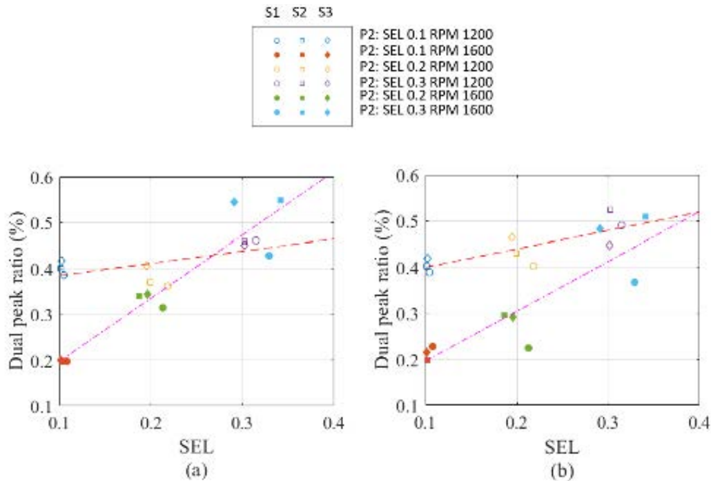
Figure 3. Dual peak ratio plotted over SEL for trials on plate 002 for normal (a) and shear force (b). Each trial is represented by a separate colour, sample points 1-3 in each trial are represented by circle, square and diamond shapes respectively, trials at 1200 rpm are not filled in whereas trials at 1600 rpm have filled in data points. The trend lines for the 1200 rpm data points are included in red and a dashed line and the ones for the 1600 rpm data point in a pink dash-dotted line.
