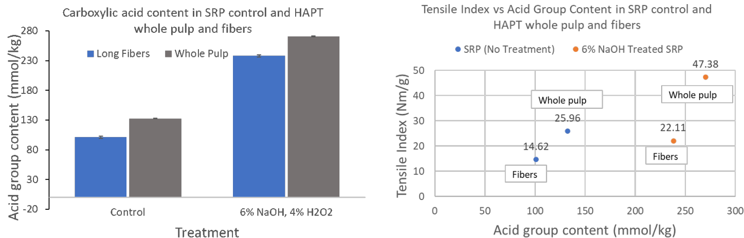
Figure 3. Carboxylic acid content of control and HAPT SRP for both the whole pulp and long fibres (left) and tensile index vs. acid group content (right)
