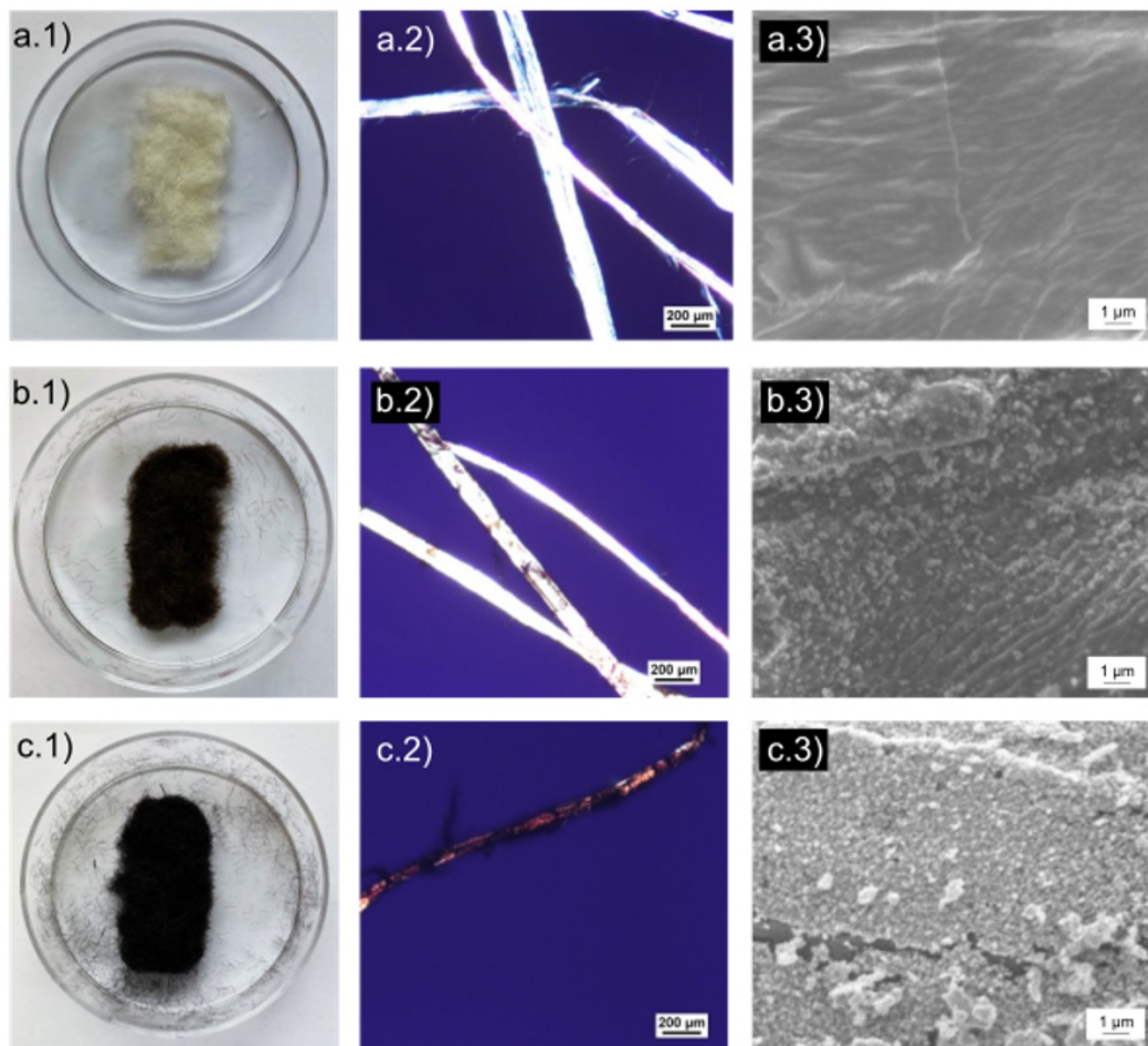
Figure 1. Images of CTMP fibres: (a) unlabelled (control), Fe-labelled fibres after (b) one and (c) four labelling steps. (a-c.1) Macroscopic view, (a-c.2) POM, and (a-c.3) SEM images showing a zoomed in area on a fibre.
