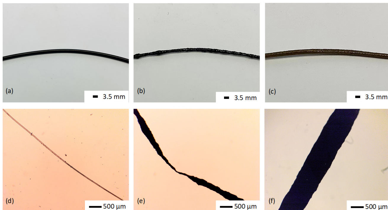
Figure 3 Images of PLA filaments without (a,d) or with fine additives (b,e) and DDSA fine additives (c,f).
