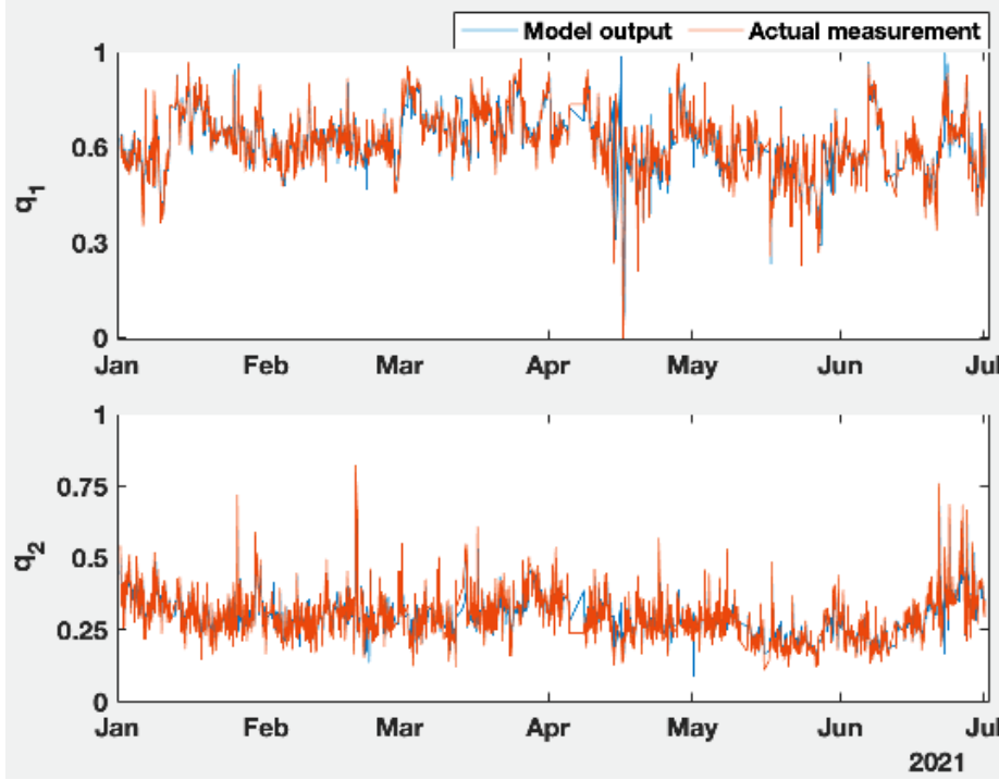
Figure 2. Model validation performance of the two selected pulp properties after normalization.
