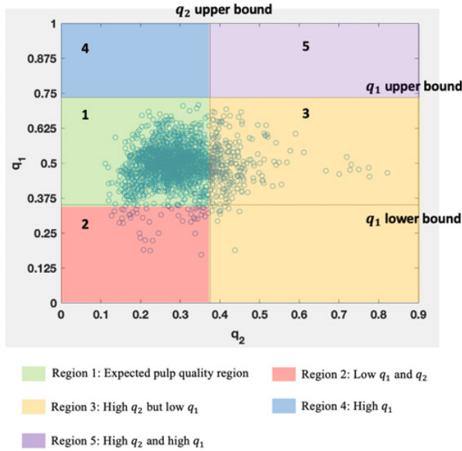
Figure 3. An illustration of pulp quality region segmentation
