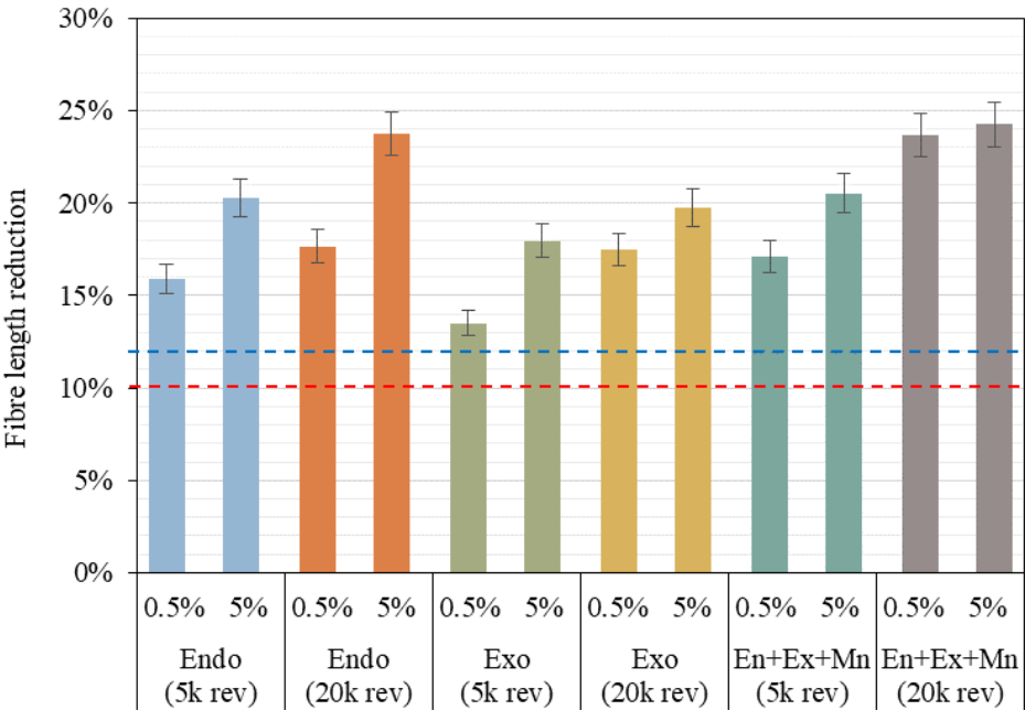
Figure 6. Effect of enzyme dosage and refining level on fibre length reduction, relative to untreated fibres, measured by FQA. The red dashed line indicates the result of refining at 5,000 revolutions, and the blue dashed line indicates refining at 20,000 revolutions, both without enzymatic hydrolysis.
