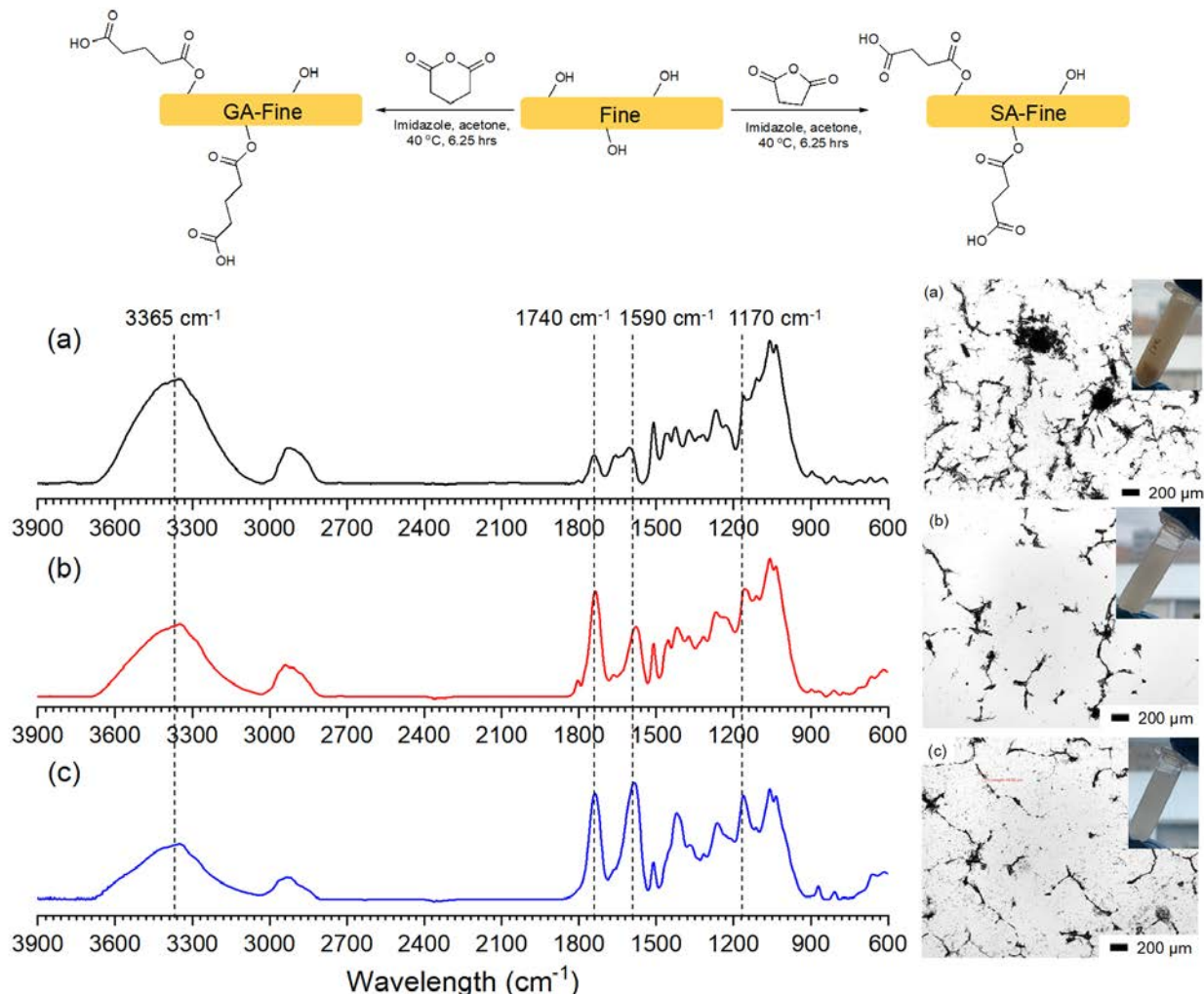
Figure 1 Reaction scheme (top) of the N-succinylimidazole esterification using glutaric anhydride and succinic anhydride; the FTIR spectra for (bottom left) of untreated fine (a), SA-fine (b), and GA-fine (c); the microscopy image (bottom right) of untreated fine (a), SA-fine (b), and GA-fine (c) and their dispersibility in the water.
