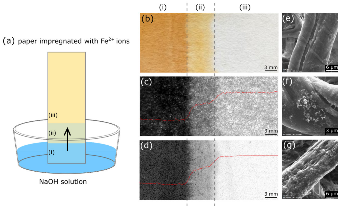
Figure 3. Liquid flow through paper as revealed by iron oxide nanoparticles, showing three regions: (i) nanoparticles precipitated on fibres by immersion in NaOH solution; (2) nanoparticles precipitated by the liquid front (NaOH solution), (iii) fibres with no contact with NaOH solution. (a) schematic representation of the test; (b) macroscopic view of paper strip with iron oxide nanoparticles; (c) image from transmitted light; (d) image from reflected light. Red curves represent the average grey scale at each region. SEM images from fibres in the regions: (e) i; (f) ii; and (g) iii.
