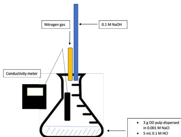
Figure 1. Acid group analysis apparatus
