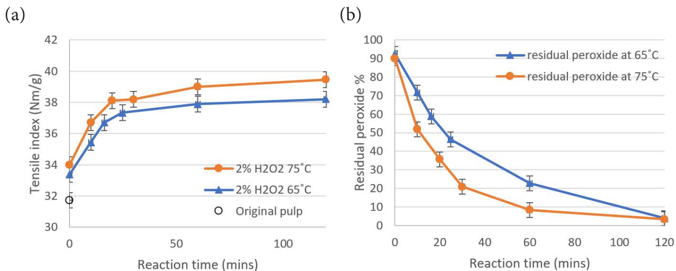
Figure 5. (a) Tensile strength as a function of HAPT time at 65°C (blue triangles) and 75°C (orange circles). (b) Residual peroxide (wt%) as a function of reaction time
