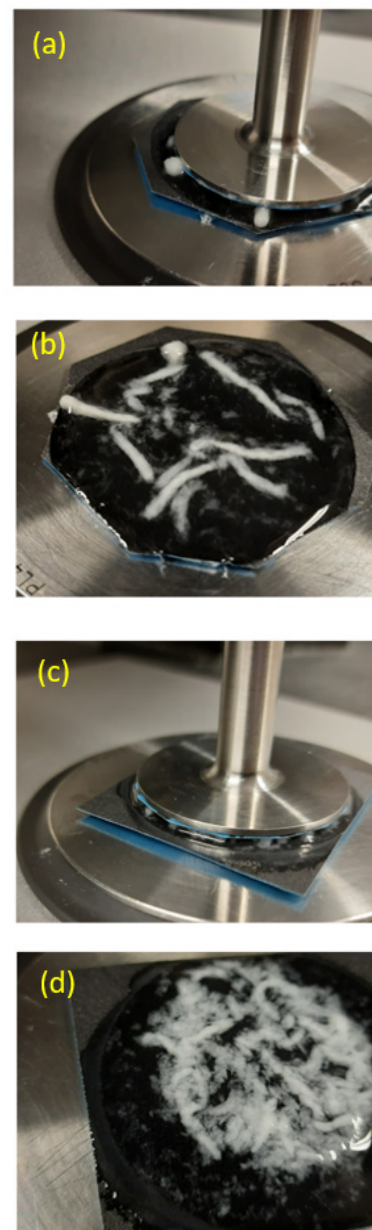
Figure 4. Formation of flocs after constant shear at 0.8 s^{-1} for 15 minutes. Suspension consistency was 1 wt%: (a), (b) Unrefined short fibres (0 kWh/ton SRE); (c), (d) MFC-like material (991 kWh/ton SRE).
