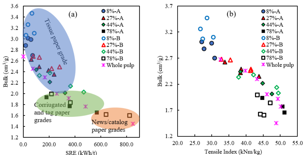
Figure 1. Relationship of a) bulk-SRE, b) bulk-tensile index for all composites; the percentage indicates the accept (short fibre) fraction in the composite
