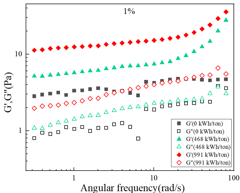
Figure 5. Angular frequency dependent storage modulus ( G' ) and loss modulus ( G'' ) at a constant shear strain 0.5% for fibre suspensions (1 wt% consistency) with different levels of SRE.
