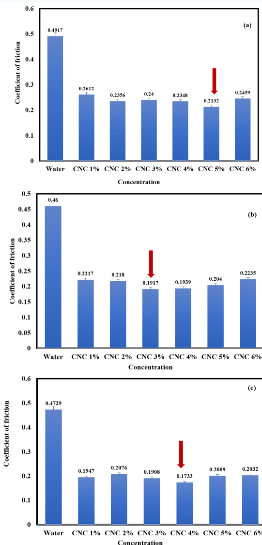
Figure 2 a-c Steady state coefficient of friction under different loads of (a) 2.5 N, (b) 7.5 N and (c) 12.5 N. The red arrows indicate the concentration where the minimum coefficient of friction occurs.
